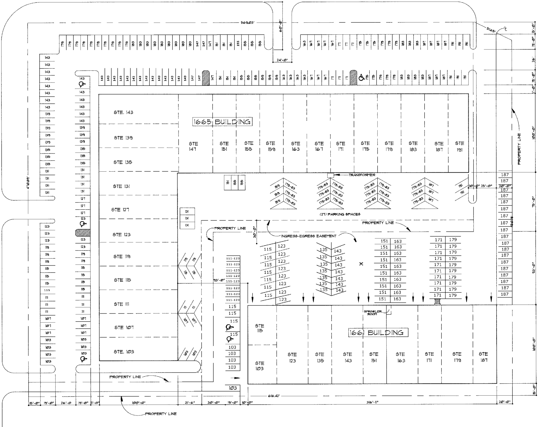
PARKING LAYOUT PLAN SCALE 1" = 30'-0"
